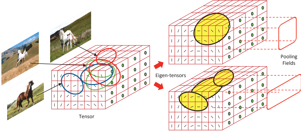
Figure 2: Receptive field learning. An image class defines an energy distribution in tensor space. An eigen-tensor decomposition produces the collection of tensor basis functions that best approximate this energy distribution. Discriminant pooling windows can be obtained from these eigentensors.
