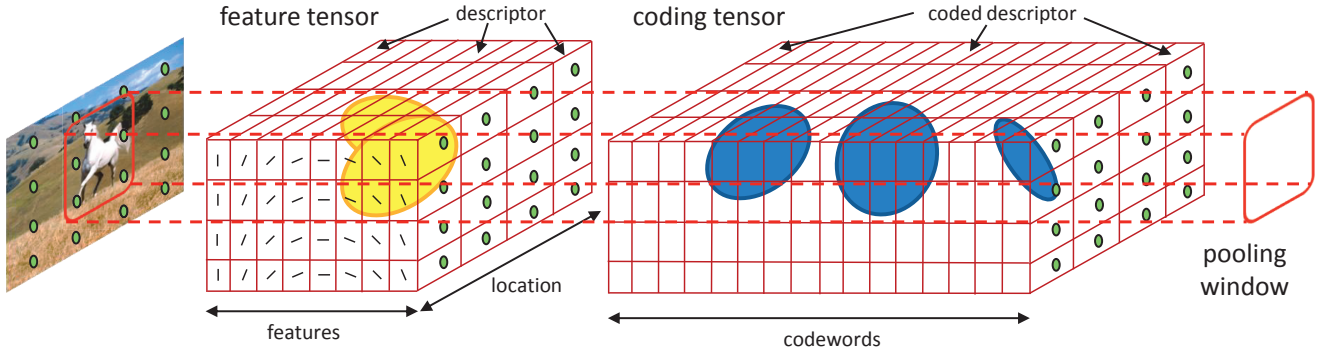
Figure 1: Under SPM, an image is first mapped into a tensor of feature (descriptor) responses and subsequently into a tensor of coding coefficients. Discriminant class information is coded as blobs of energy within these tensors. Discriminant pooling windows can be recovered by detecting the eigenblobs of tensor response to images of the class.
