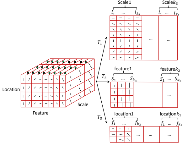
Figure 3: The three possible flattenings, \mathbf{T}_i, i = \{1, 2, 3\} of the tensor of feature responses.
